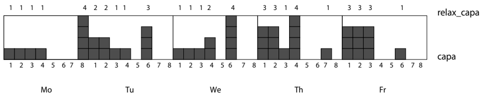
Fig. 2. Over-loads in the solution of Example 3.1.
