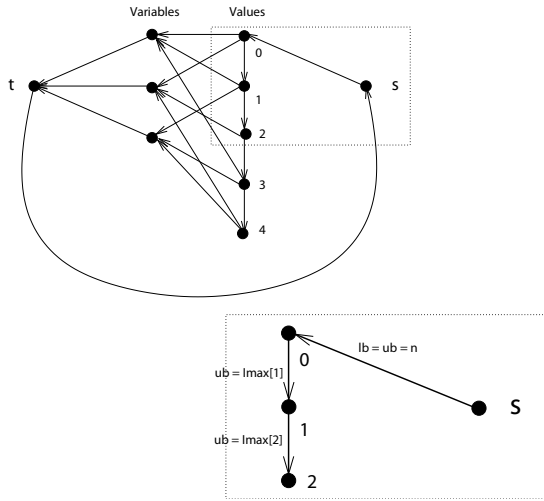
Fig. 3. Example of a digraph representing an ORDEREDDISTRIBUTE( X, T, I_{max} ). Arcs between values and variables have a lower bound equal to 0 and an upper bound equal to 1.
